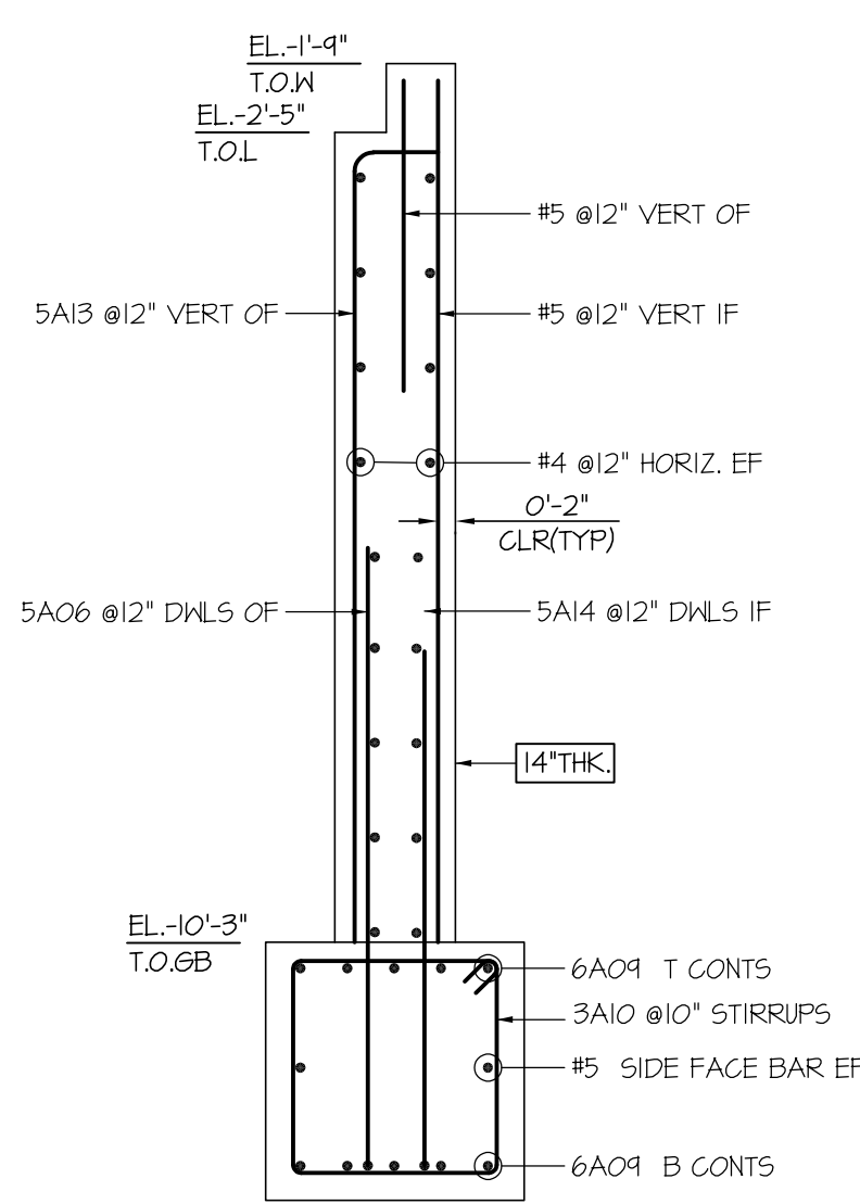
SECTION 2 SCALE: 1/2" = 1'-0" (GB1=2'-6"x2'-6")
