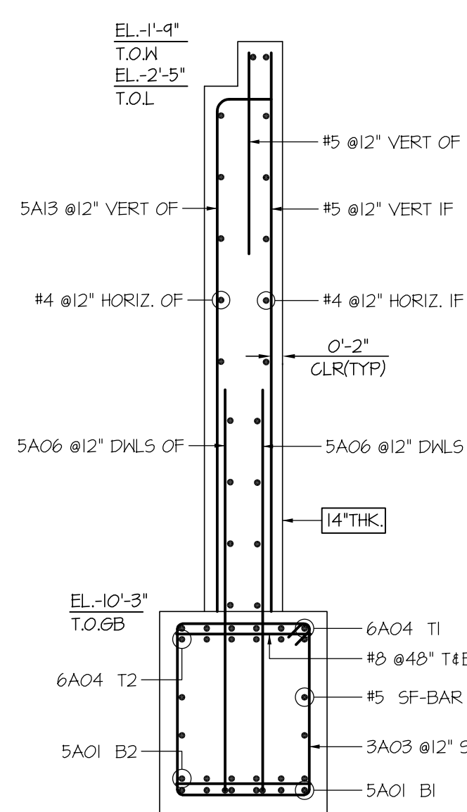
SECTION 1 SCALE: 1/2" = 1'-0" (GB4=2'-6"x3'-0")
