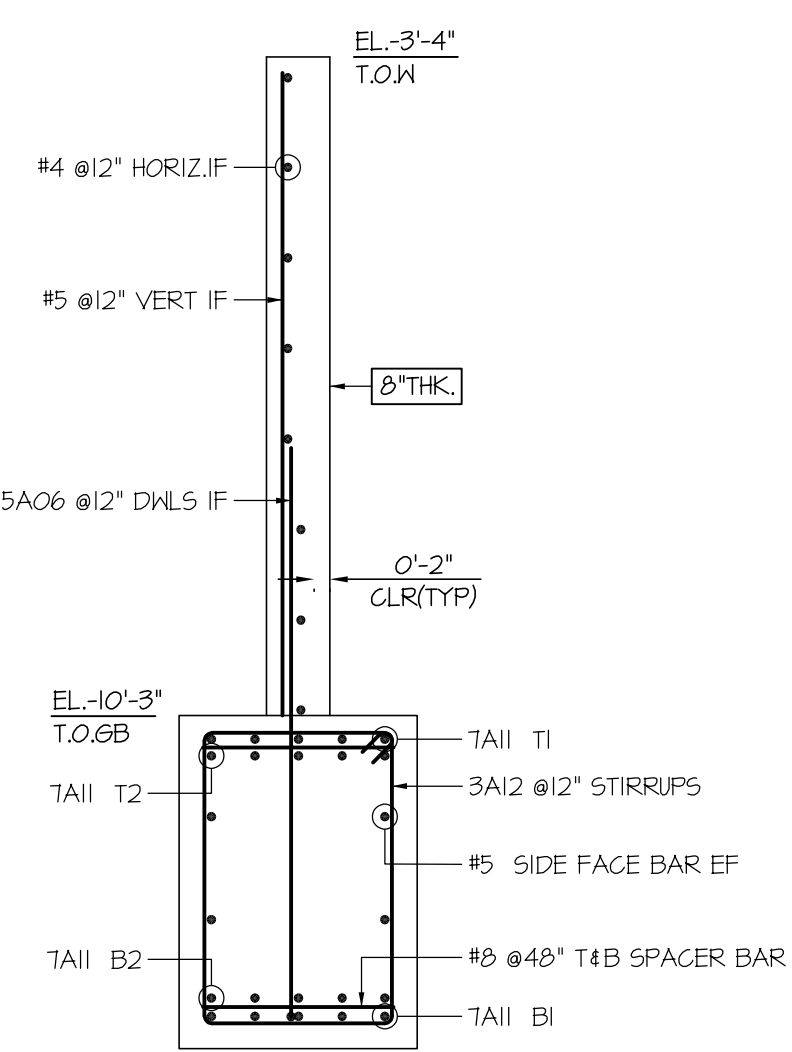
SECTION 3 SCALE: 1/2" = 1'-0" (GB2=2'-6"x3'-6")
